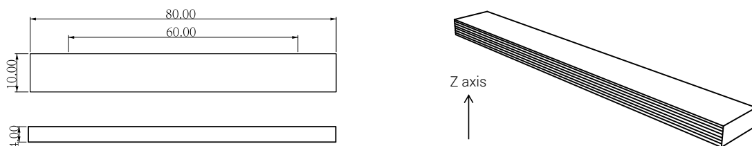
Fig 2. Flexural testing specimen
