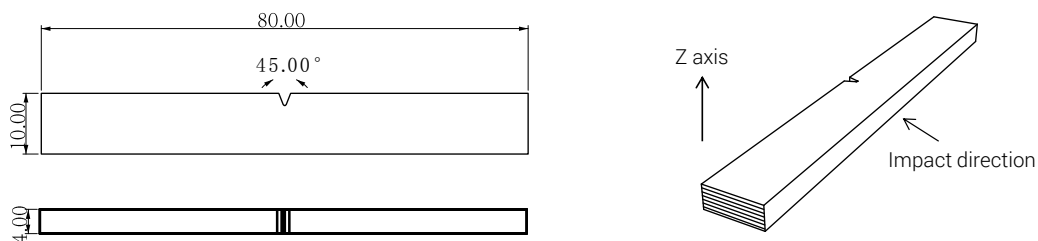
Fig 3. Impact testing specimen
